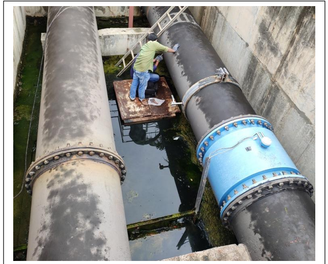
1000mm Electro Magnetic Flow meter Calibration.
