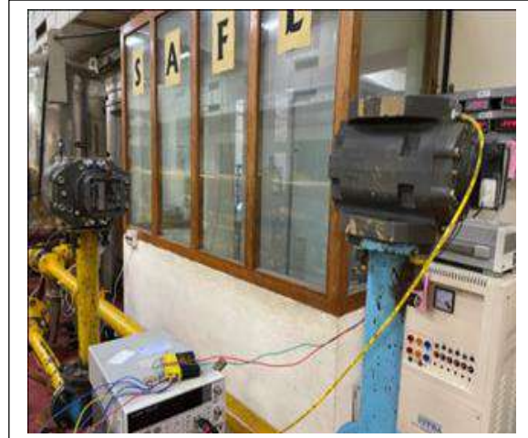
Calibration of flow meters at Air Flow Laboratory
